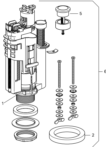
Flushing Valve Type 280* Single-flush
