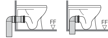
A. Floor-Mount Rear Discharge into Wall B. Floor-Mount Rear Discharge into Floor
