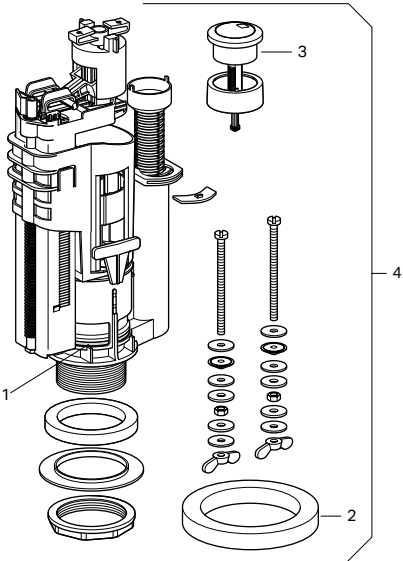
Flushing Valve Type 280* Dual-flush
